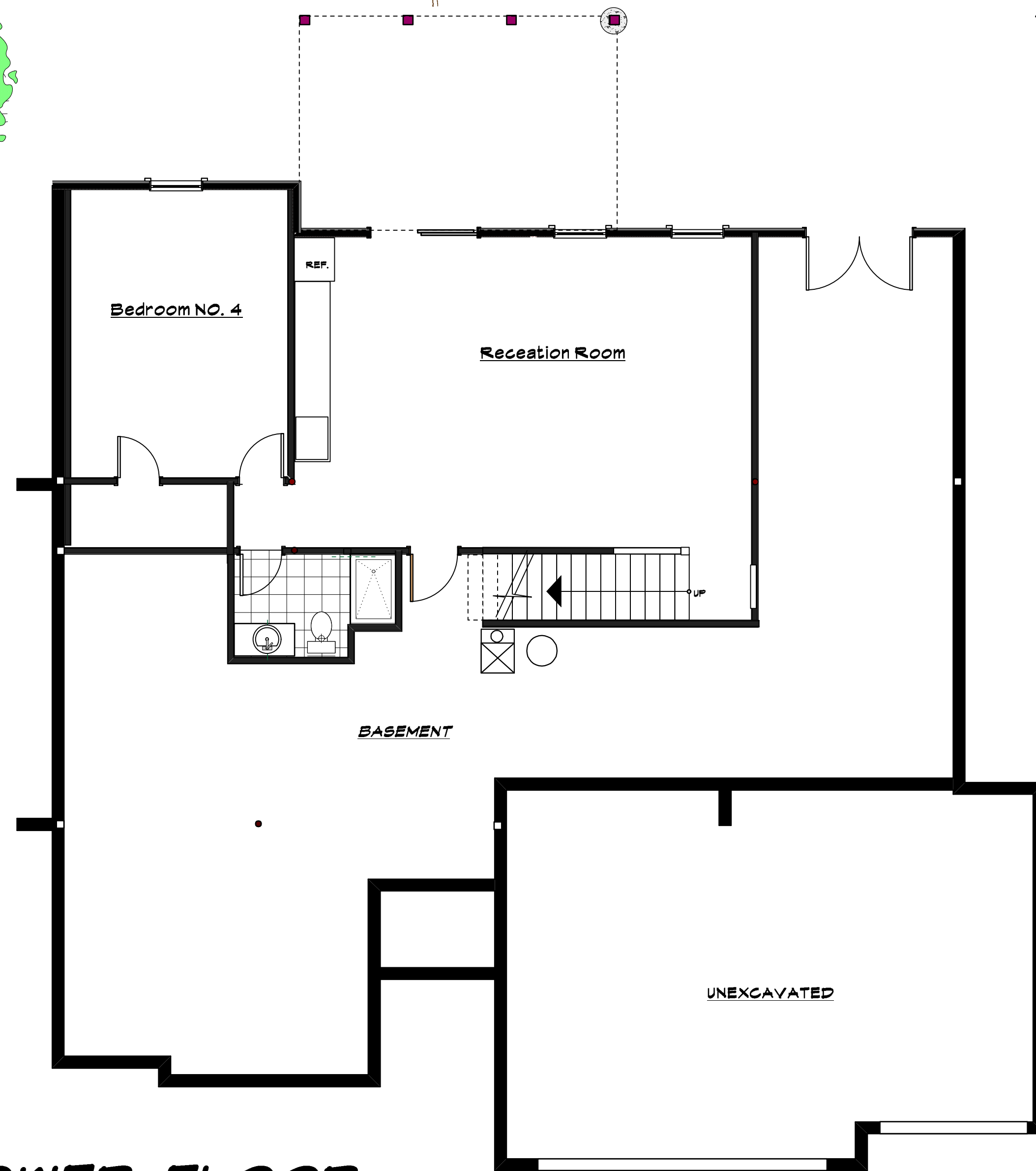
LOWER FLOOR
